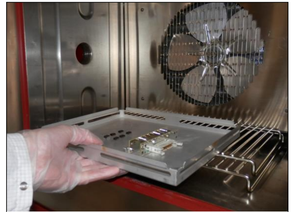
Set-up of the components in the climatic chamber
